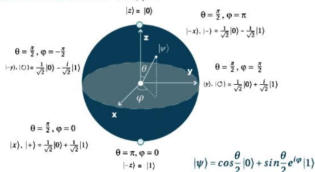
Qubit na esfera de Bloch \theta = 0, \varphi = 0
